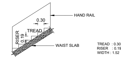
STAIRCASE DETAILS SCALE 1:100
