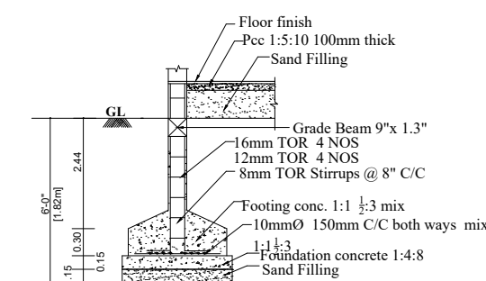
FOUNDATION DETAILS
