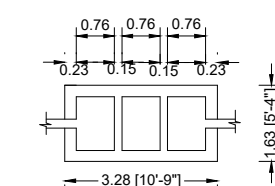
SEPTIC TANK DETAILS SCALE 1:100
