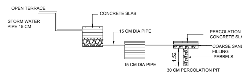
RAINWATER HARVESTING SYSTEM NOT TO SCALE
