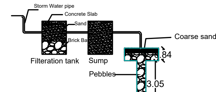
CONSTRUCTION DETAILS OF RECHARGE TRENCH
