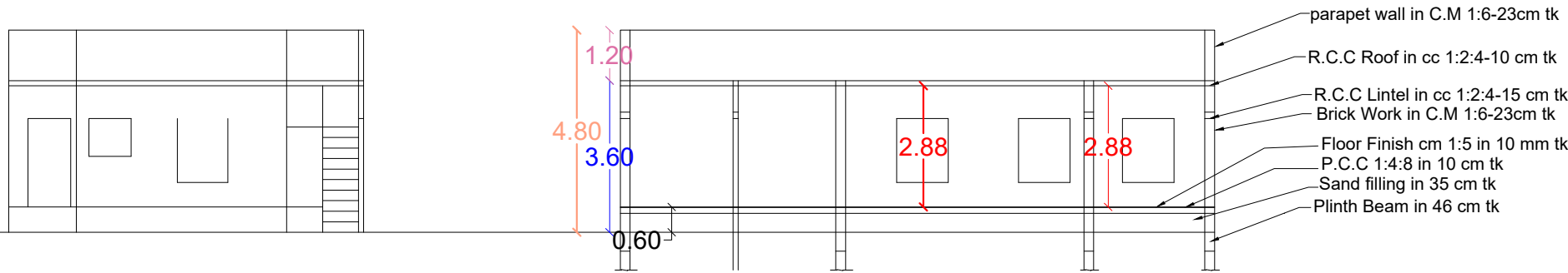
FRONT ELEVATION
