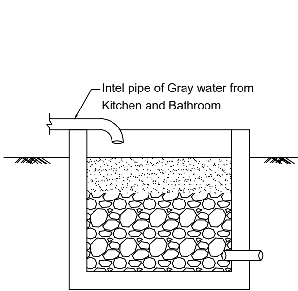
GREY WATER RECYCLING CHAMBER:-
