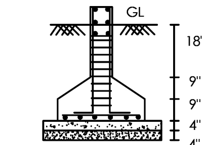
FOUNDATION DETAILS
