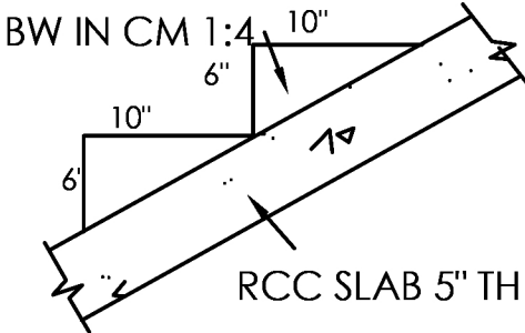
STAIR DETAIL
