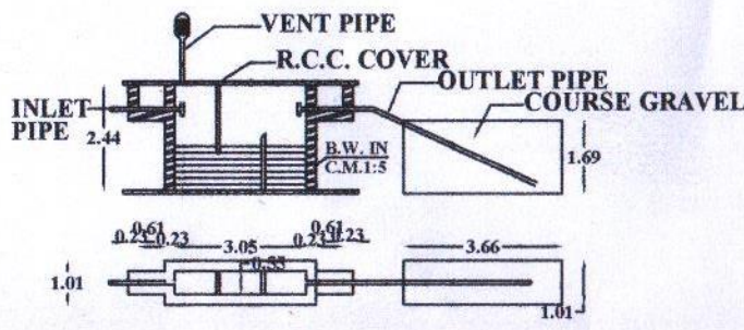
SEPTIC TANK & OF DISPERSION TRENCH DETAILS
