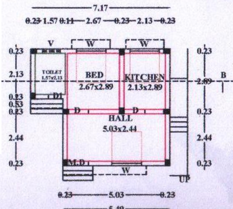
FLOOR-GROUND
