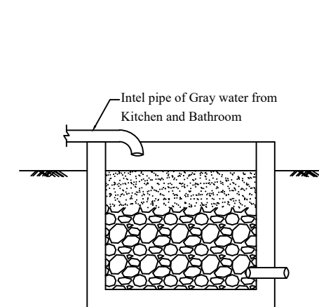
GREY WATER RECYCLING CHAMBER:-
