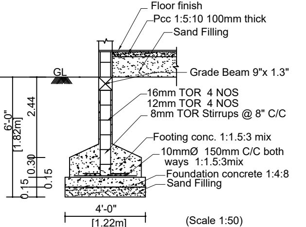
FOUNDATION DETAILS
