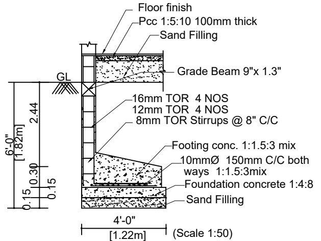
FOUNDATION DETAILS
