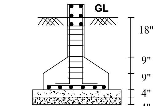
FOUNDATION DETAILS
