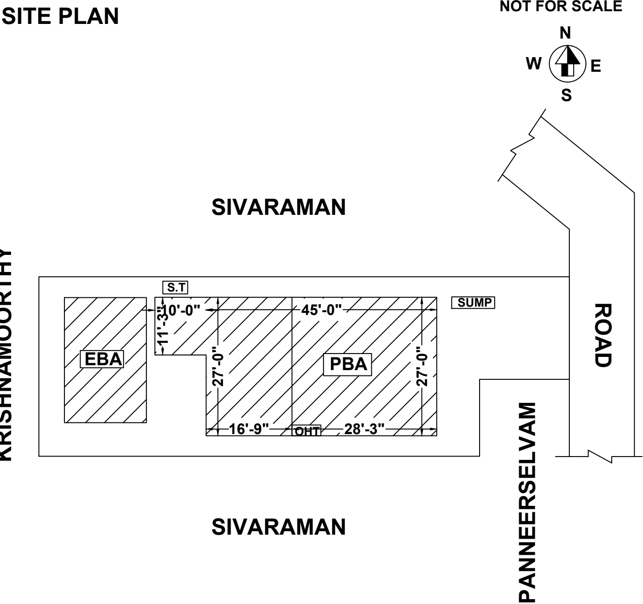
SITE PLAN
