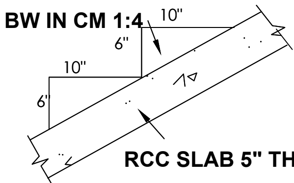
STAIR DETAIL
