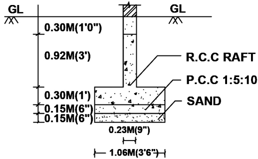
"FOUNDATION DETAILS" SCALE - 1:50
