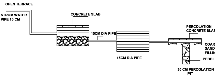
RAIN WATER HARVESTING SYSTEM
