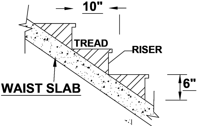
" STAIRCASE DETAIL(NTS)"
