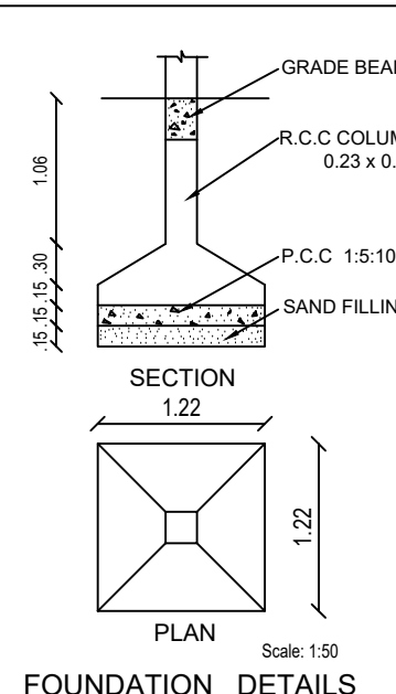
FOUNDATION DETAILS
