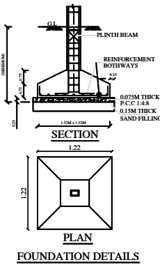
FOUNDATION DETAILS
