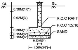
"FOUNDATION DETAILS" SCALE - 1:50
