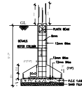
FOUNDATION DETAILS SCALE : 1:50.
