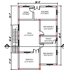
PRO. GROUND FLOOR PLAN
