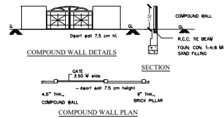
COMPOUND WALL PLAN
