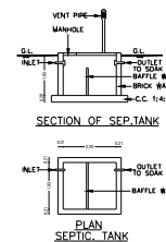
PLAN SEPTIC TANK
