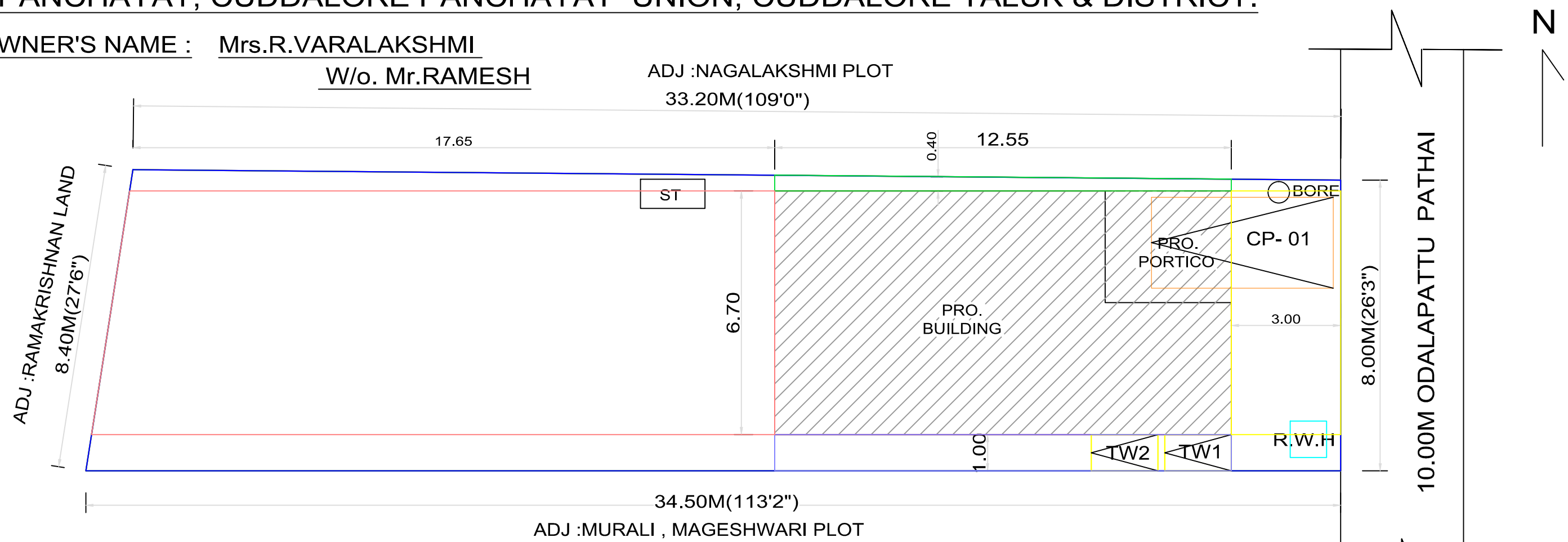
SITE PLAN
