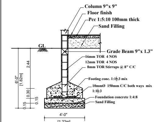
FOUNDATION DETAILS (SCALE 1:50)
