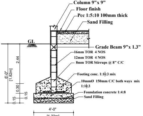
FOUNDATION DETAILS (SCALE 1:50)
