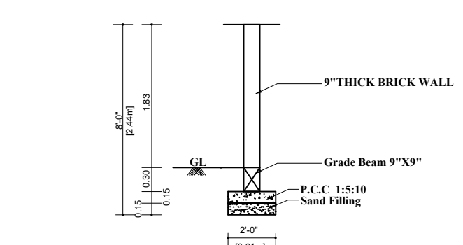
SECTION DETAIL (SCALE 1:50)
