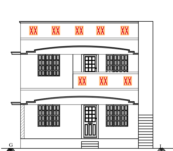
FRONT ELEVATION
