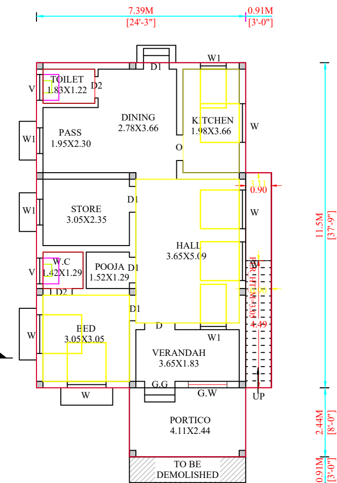
EXIS.GROUND FLOOR PLAN
