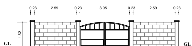
FRONT ELEVATION (SCALE 1:100)
