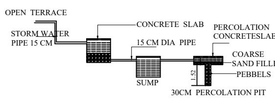
RAINWATER HARVESTING SYSTEM (SCALE - 1:200)
