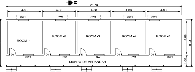
PLAN ( LABOUR'S ROOM ) ( BLOCK -II )
