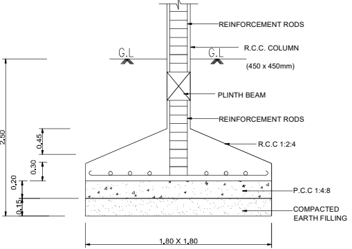
FOUNDATION DETAILS
