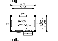
PLAN ( SECURITY ROOM ) BLOCK - V
