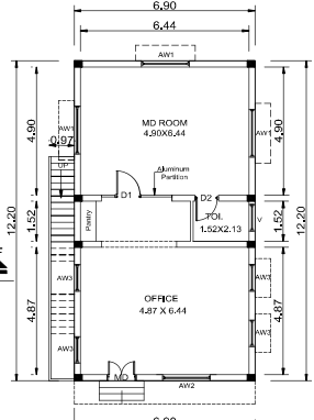
PLAN ( OFFICE ) ( BLOCK -VI )
