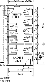
PLAN ( LABOUR'S TOILET ) ( BLOCK -III )
