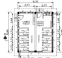
PLAN ( STAFF TOILET ) - BLOCK - IV
