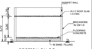
SECTION ON GG
