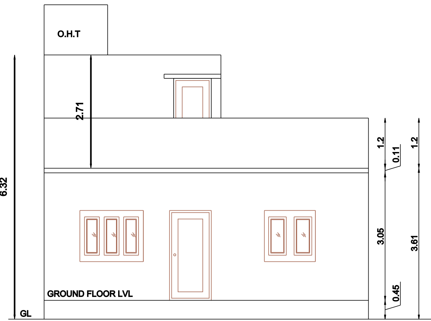
FRONT ELEVATION
