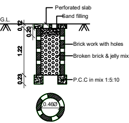
PERCOLATION PIT FOR 30 Sq. m. (Scale:- 1:50)
