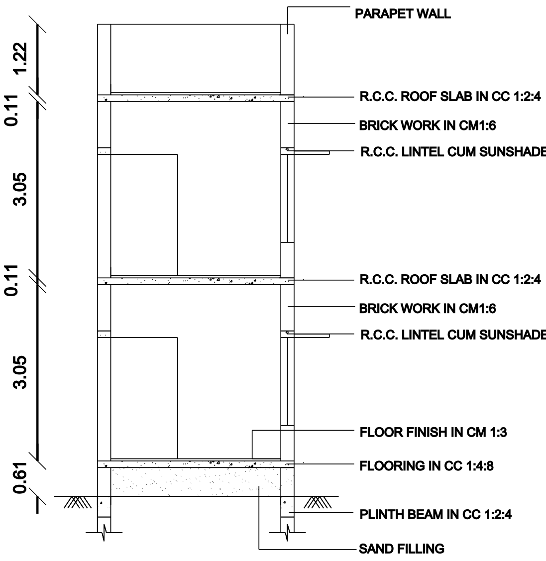
SECTION ON 'FB'
