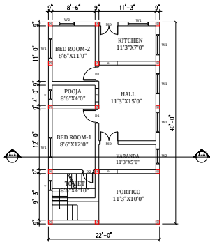
PRO. GROUND FLOOR PLAN
