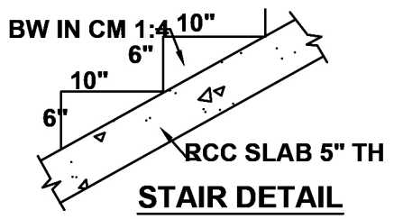
STAIR DETAIL
