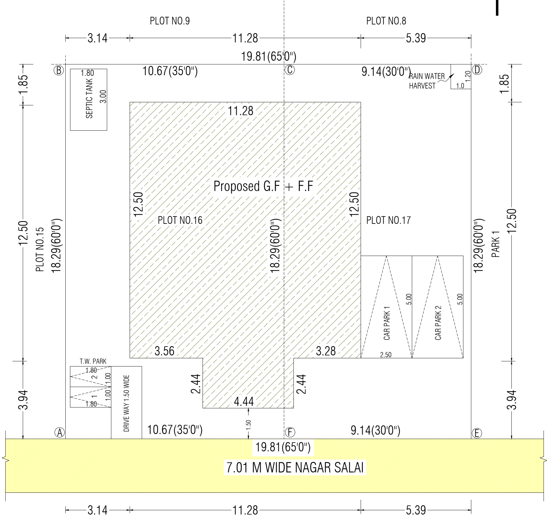
SITE PLAN
