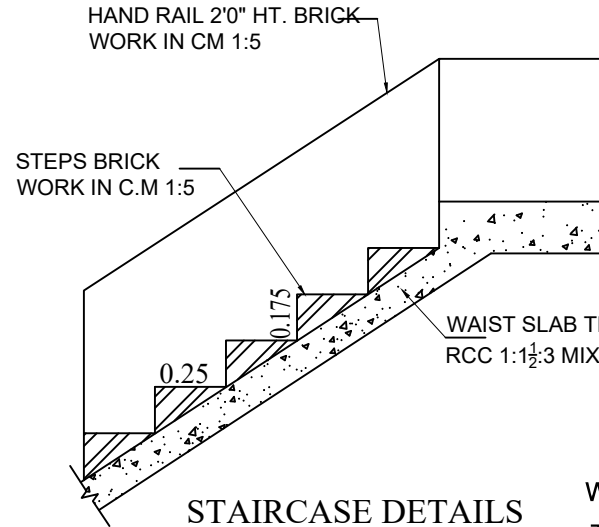
STAIRCASE DETAILS
