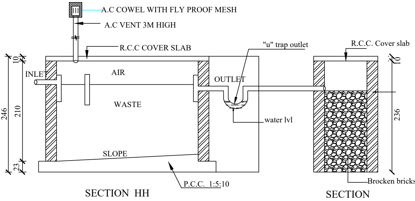
SECTION HH
