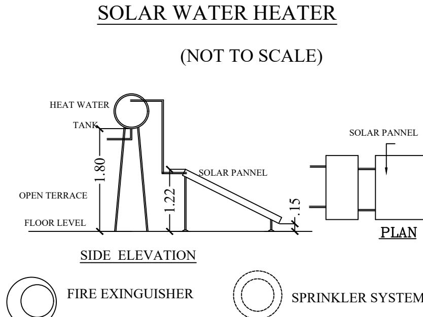
SOLAR WATER HEATER
