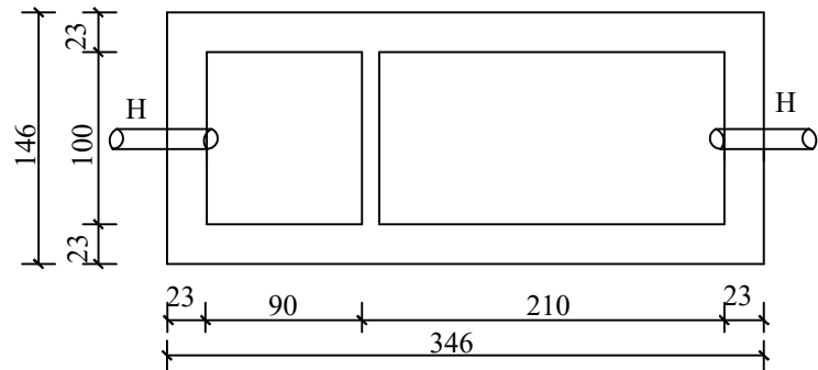
PLAN SEPTIC TANK DETAILS
