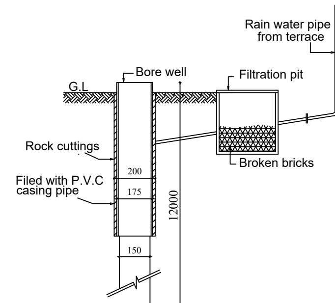
RAIN WATER HARVESTING DETAIL
