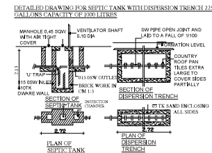
DETAILED DRAWING FOR SEPTIC TANK WITH DISPERSION TRENCH 2/15
