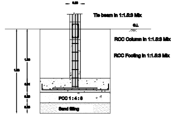
COLOUMN FOUNDATION DETAILS
