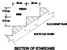
SECTION OF STAIRCASE
