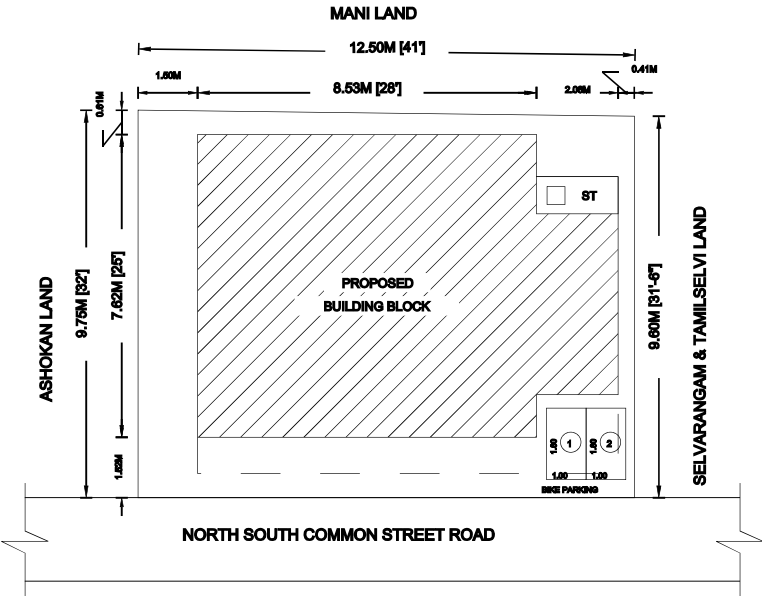
SITE PLAN
