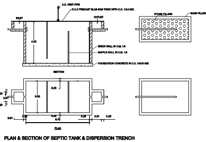
PLAN & SECTION OF SEPTIC TANK & DISPERSION TRENCH
