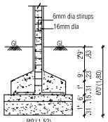
FOUNDATION DETAIL SCALE (1:50)
