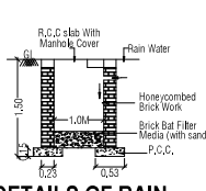
DETAILS OF RAIN WATER COLLECTION PIT SCALE:- 1" = 4'0"
