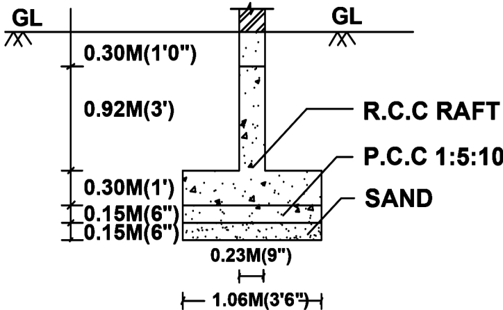
"FOUNDATION DETAILS"
