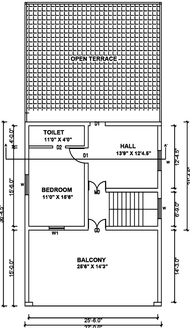
FIRST FLOOR
