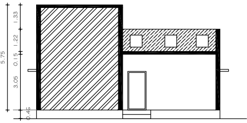
FRONT ELEVATION.
