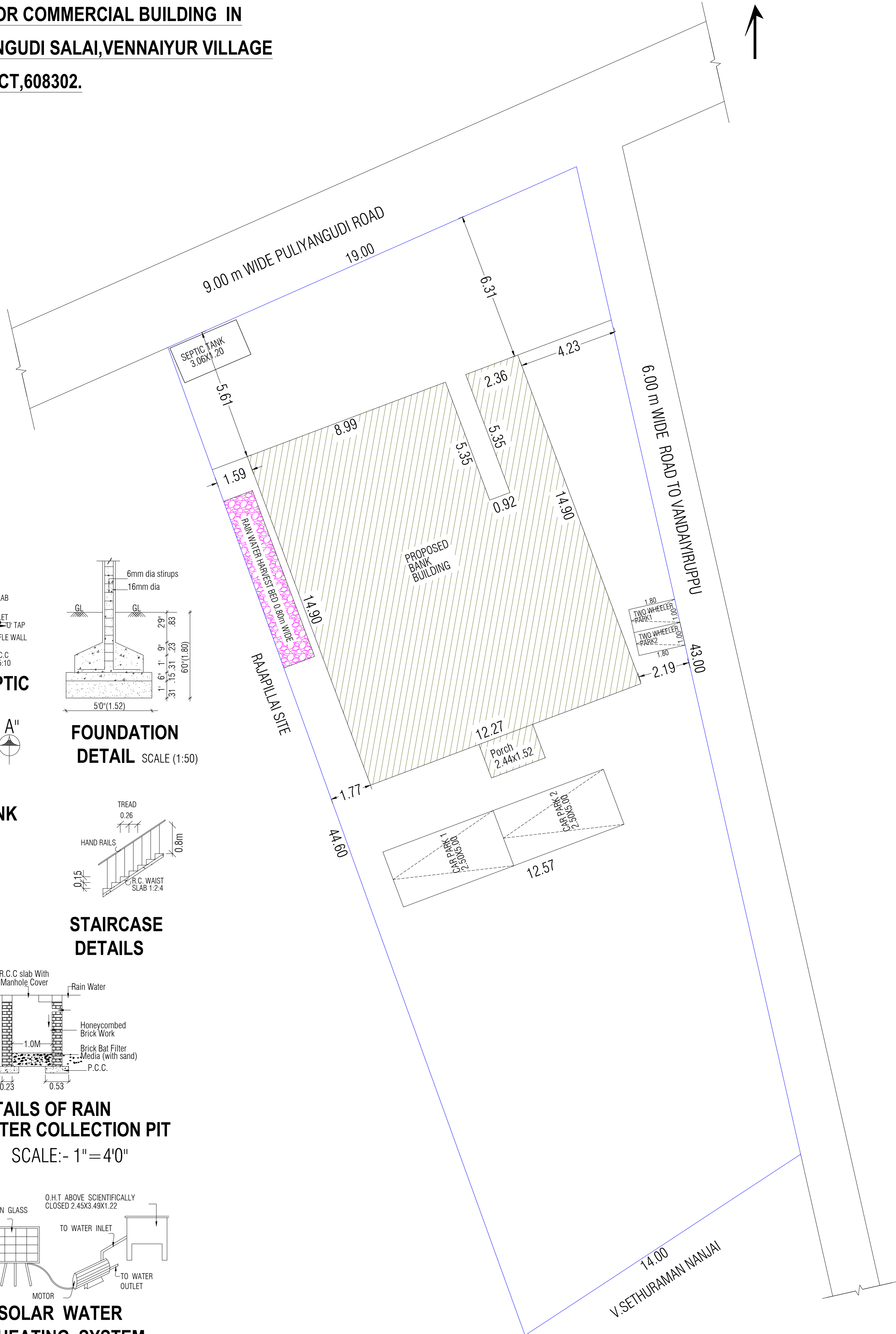
SITE PLAN
