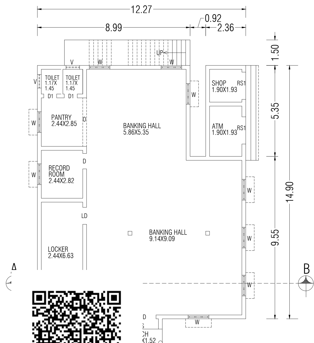
ND FLOOR PLAN
