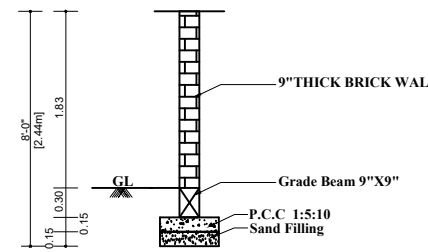
SECTION DETAIL (SCALE 1:50)
