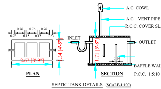
SEPTIC TANK DETAILS (SCALE:1:100)
