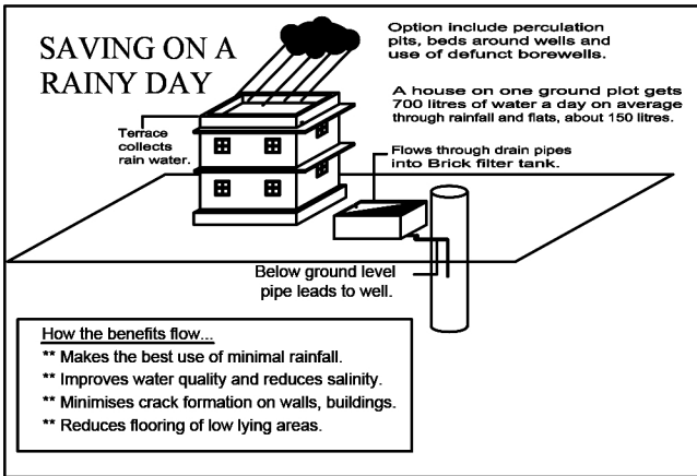
WELL AND RAIN WATER STORAGE DETAILS
