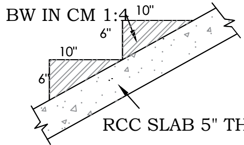
STAIR DETAIL
