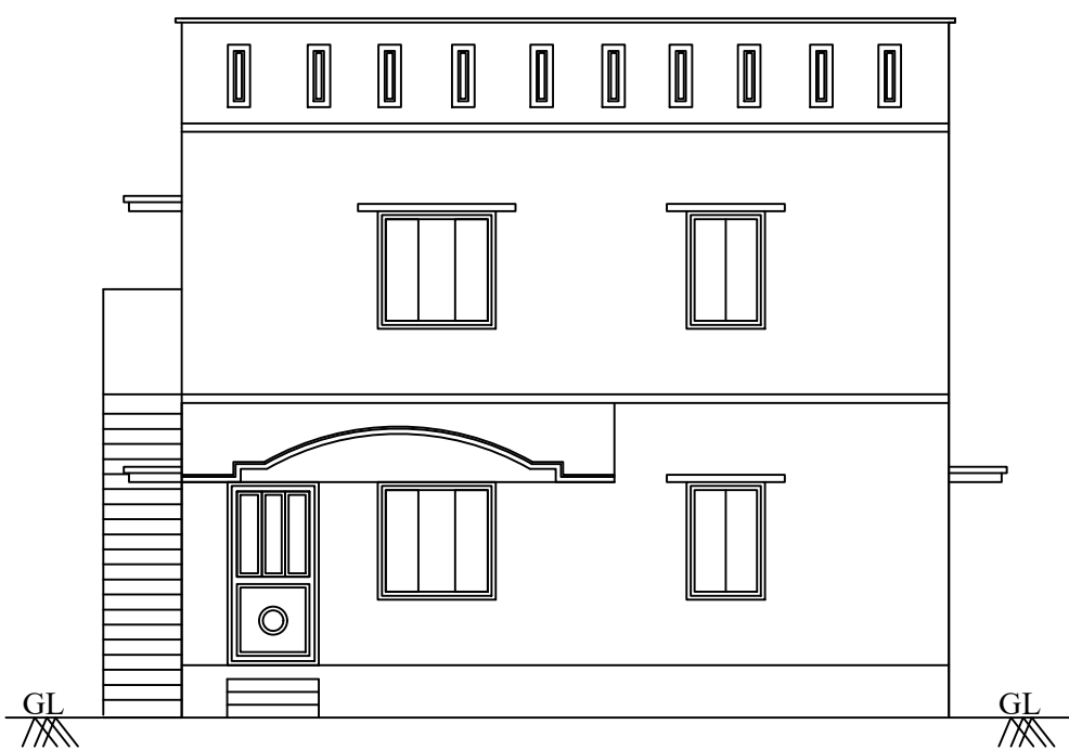
FRONT ELEVATION
