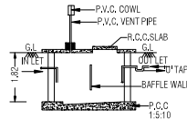
SEC. OF SEPTIC TANK "AA"
