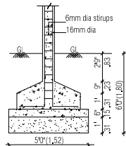
FOUNDATION DETAIL SCALE (1:50)
