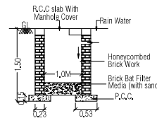
DETAILS OF RAIN WATER COLLECTION PIT SCALE:- 1" = 4'0"
