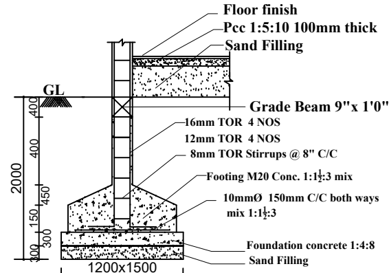
RCC COLUMN FOOTING
