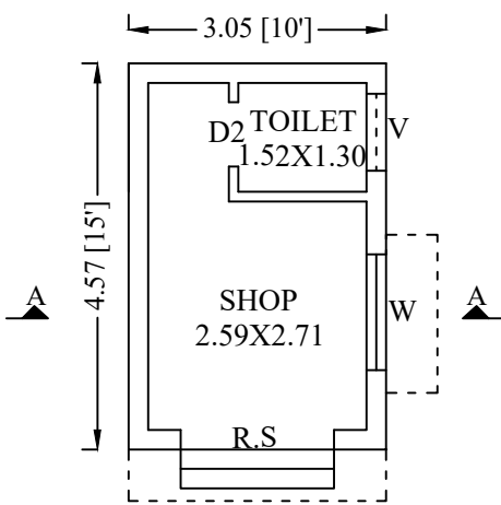
PLAN Scale-1:100
