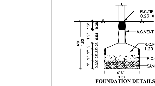
FOUNDATION DETAILS
