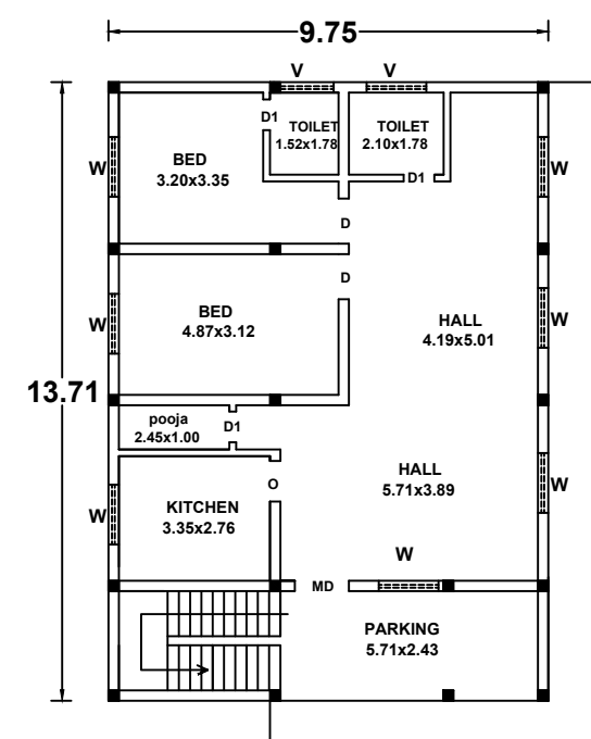
GROUND FLOOR PLAN- EAST facing
