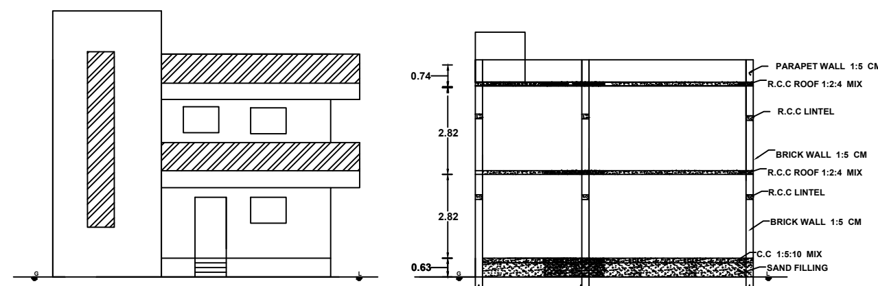
FRONT ELEVATION
