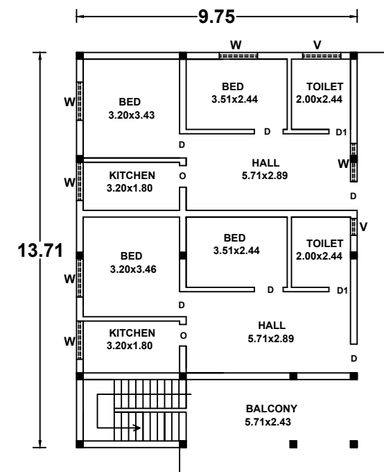
FIRST FLOOR PLAN- North facing
