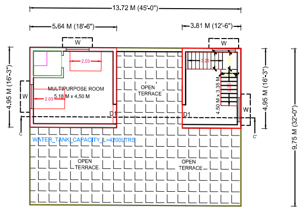
SECOND FLOOR & HEADROOM PLAN
