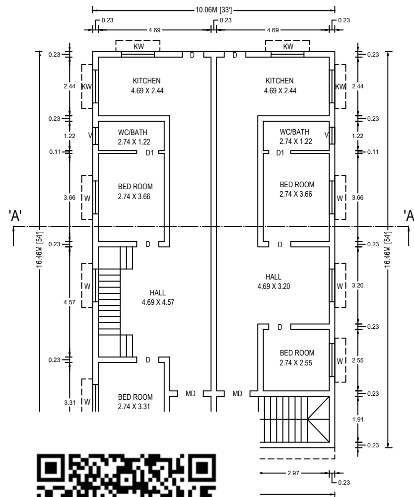
FLOOR PLAN
