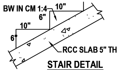
STAIR DETAIL
