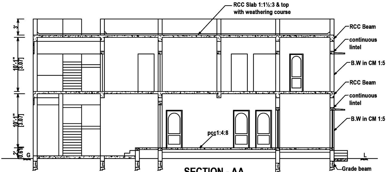
SECTION - AA
