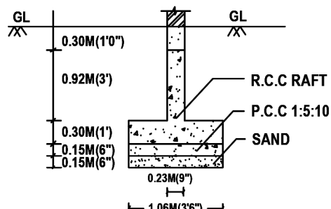
"FOUNDATION DETAILS"
