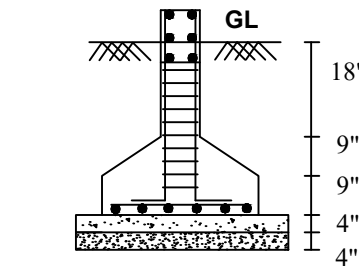
FOUNDATION DETAILS
