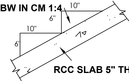
STAIR DETAIL
