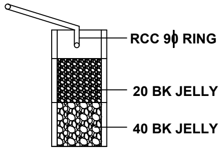
RAINWATER HARVEST PIT
