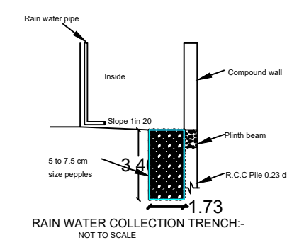
RAIN WATER COLLECTION TRENCH:- NOT TO SCALE
