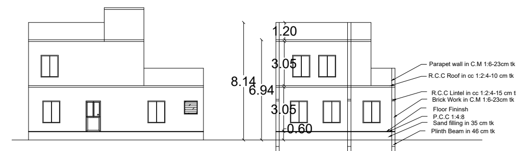
SECTION ON AR
