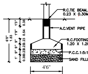
FOUNDATION DETAILS
