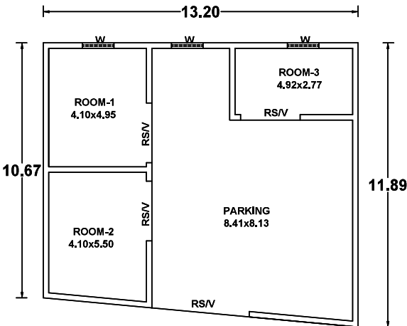
GROUND FLOOR PLAN (commercial)
