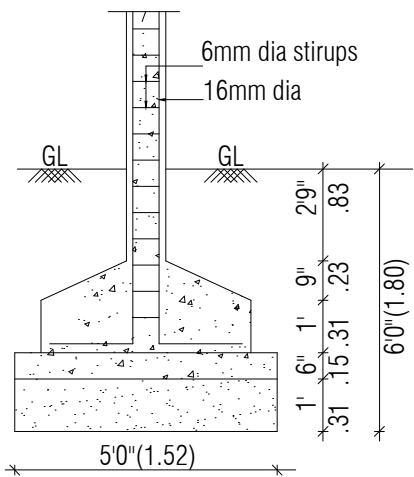
COLUMN FOUNDATION DETAIL
