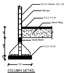
COLUMN DETAIL
