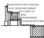
RAINWATER HARVESTING
