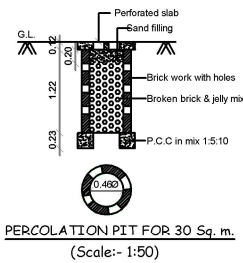
RAINWATER HARVESTING
