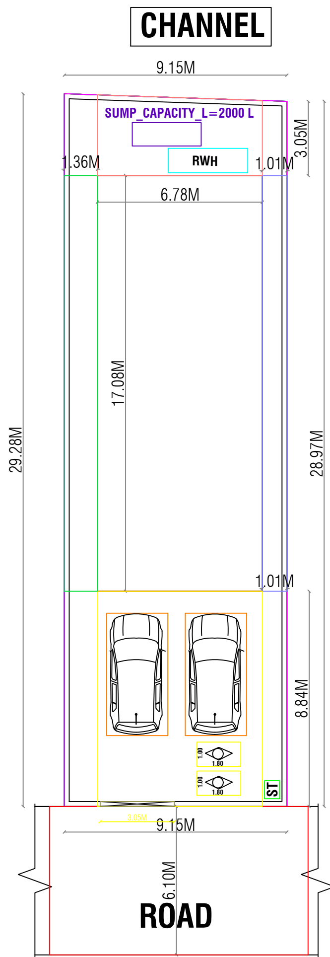
SITE PLAN
