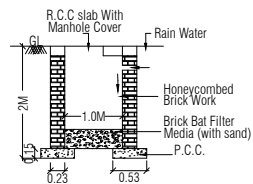
DETAILS OF RAIN WATER COLLECTION PIT SCALE:- 1"=4'0"
