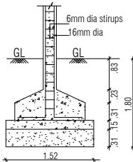
FOUNDATION DETAIL
