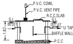
SEC. OF SEPTIC TANK"AA"
