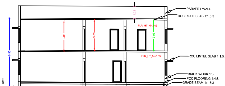
SECTION AA' & BB'
