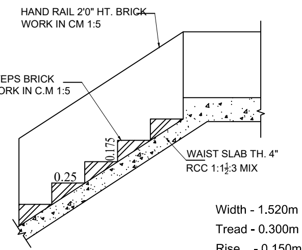
STAIRCASE DETAILS Scale (1:50)
