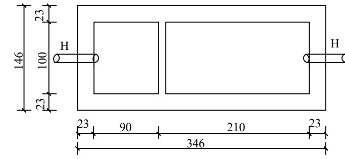
PLAN SEPTIC TANK DETAILS (SCALE: 1:50)
