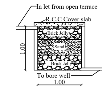
RAIN WATER HARVEST PIT
