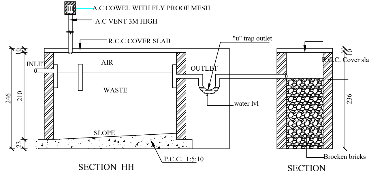
SECTION HH
